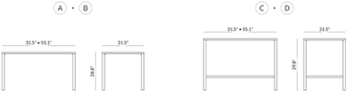
Moontable: A and B the low tables, C and D the high tables. Technical drawing reproduced from the 2026 Listino Urbantime. Dimensions are in inches; inch equivalents are given above.
