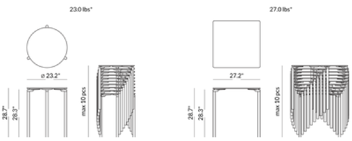
LEG.03 (round, A) and LEG.04 (square, B), with stacking. Technical drawing reproduced from the 2026 Listino Urbantime. Dimensions are in inches; weights in pounds.
