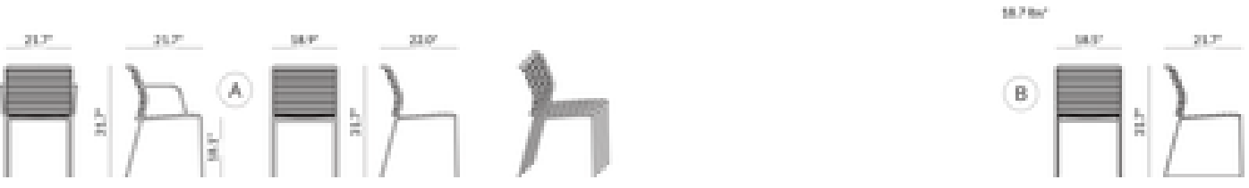
Libra Wire: A the 4-leg chair, with and without armrests; B the skid chair. Technical drawing reproduced from the 2026 Listino Urbantime. Dimensions are in inches; inch equivalents are given above.
