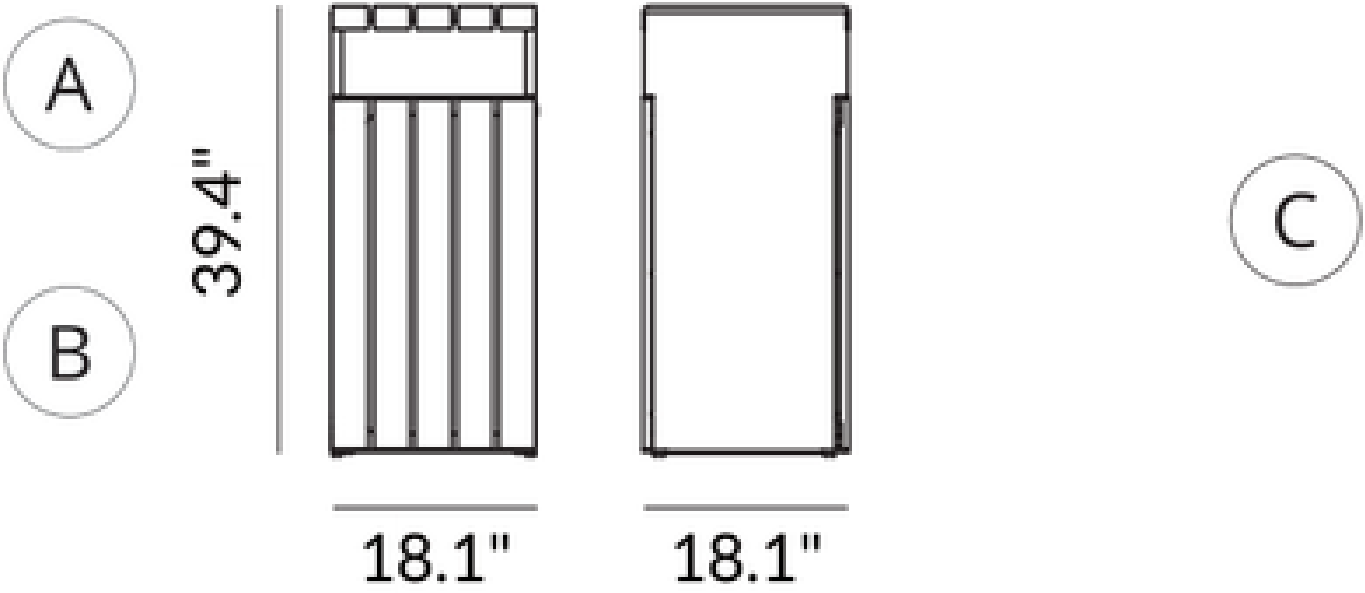
Litter bin: A basic, B with ashtray. C is the decorative planter, which shares the same shell. Technical drawing reproduced from the 2026 Listino Urbantime. Dimensions are in inches; weights in pounds.
