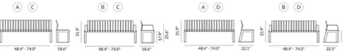
Bench with backrest, 2- and 3-seat modules. A without armrests, B with armrests; C vertical legs, D trapezium legs. Technical drawing reproduced from the 2026 Listino Urbantime. Dimensions are in inches; weights in pounds.
