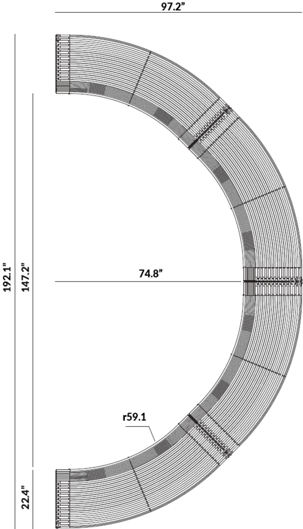
Convex Half-Circle Configuration
