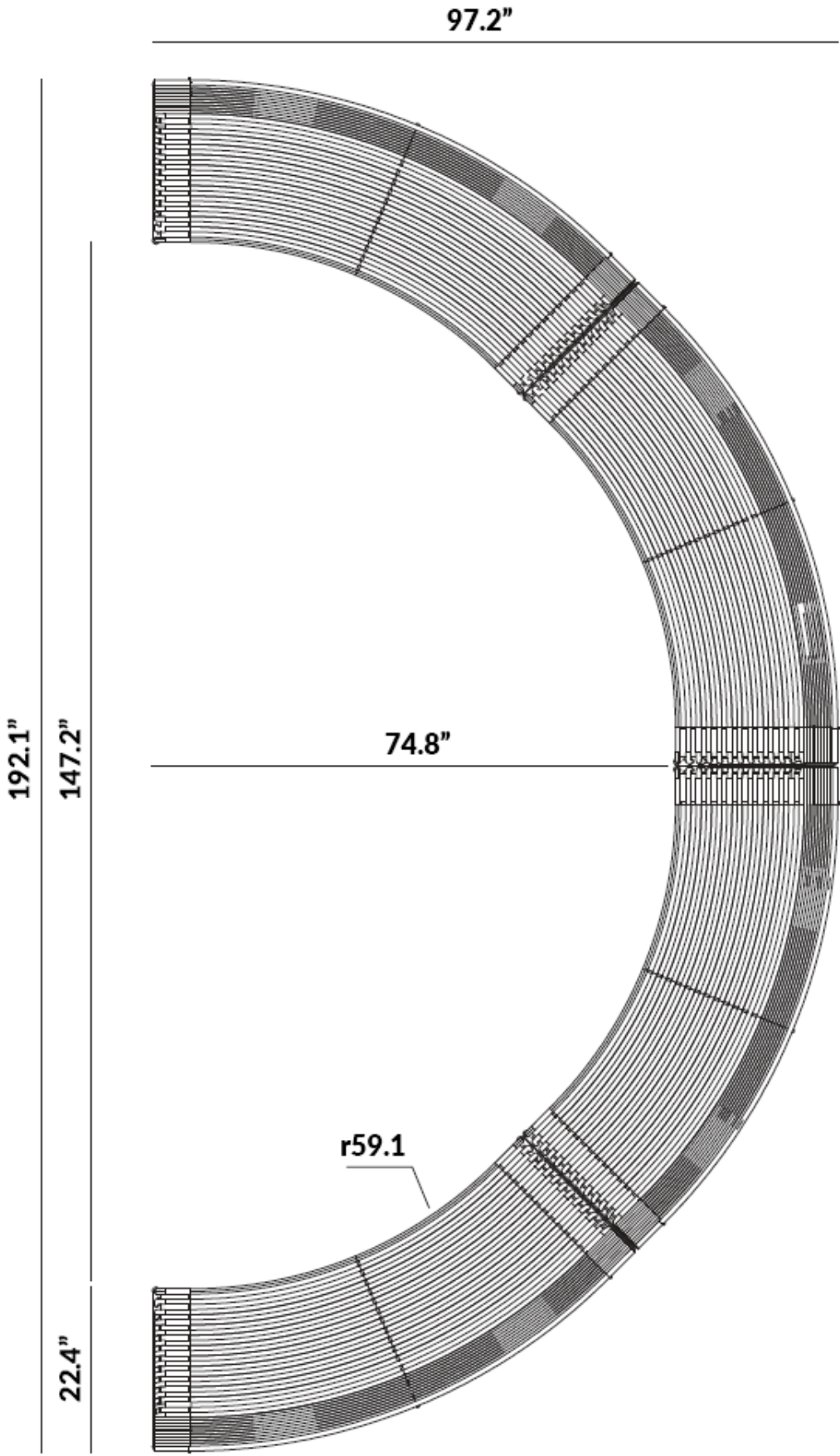
Concave Half-Circle Configuration
